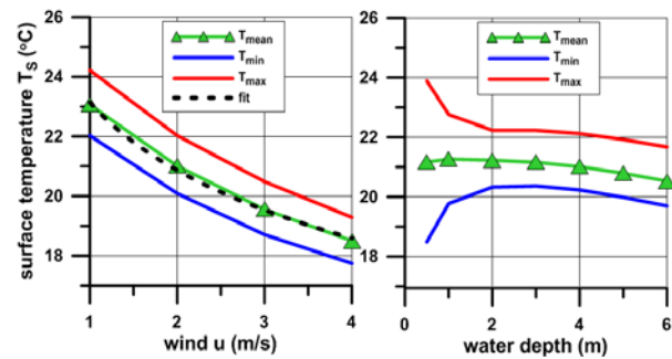
Figure 6: Sensitivity of water surface temperature for variation of wind forcing and depth of the water body.
