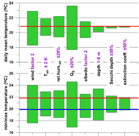
Figure 5: Sensitivity of the surface water temperature on parameter variation of the lake model.
