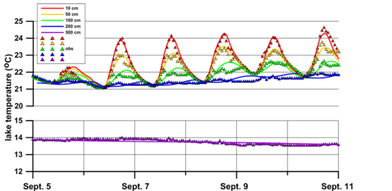
Figure 4: Above: Observed and simulated water temperatures for the centre of the Maschsee (location 1 in Figure 7). Meteorological data are given in the upper and lower panel. below: Observed and simulated water temperatures for the Kiesteich (location 2 in Figure 7).
