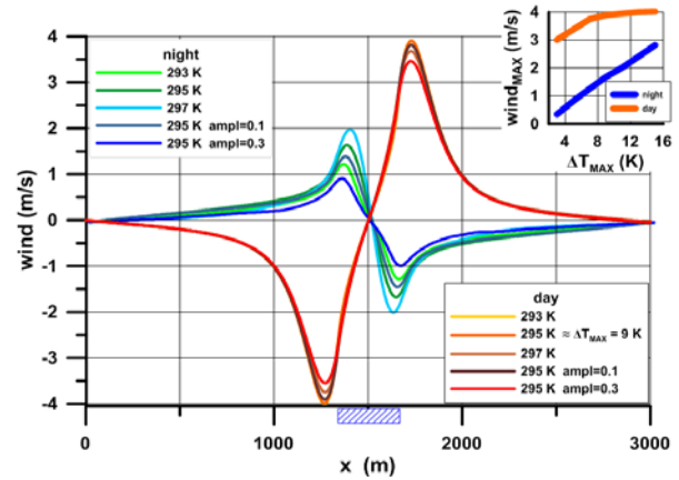
Figure 3: Simulated 10m wind for 14 hours (day) and 04 hours (night) for different water surface temperatures. Maximum wind speed for the two selected times depending on the maximum temperature difference between water and bare soil is given in the inserted graph.
