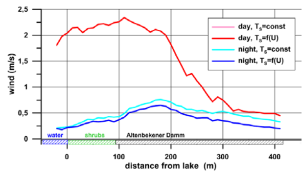
Figure 8: Simulated wind speed in 2m a.g. along the Altenbekener Damm for 14 hours (day) and 04 hours (night) for different water temperatures.
