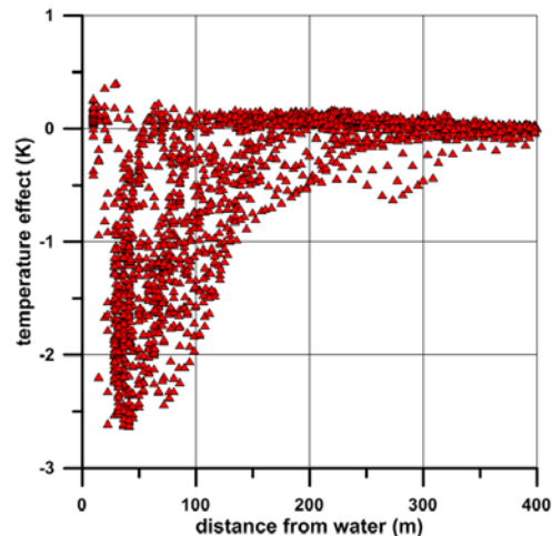
Figure 9: Temperature effect of blue spaces during daytime for grid points with landuse "street".
