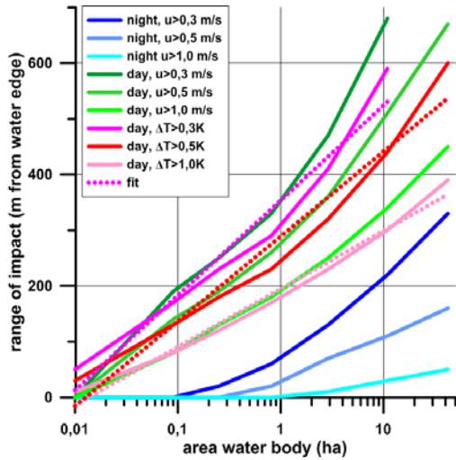
Figure 2: Simulated range of impact for various thresholds for different areas of the water body.
