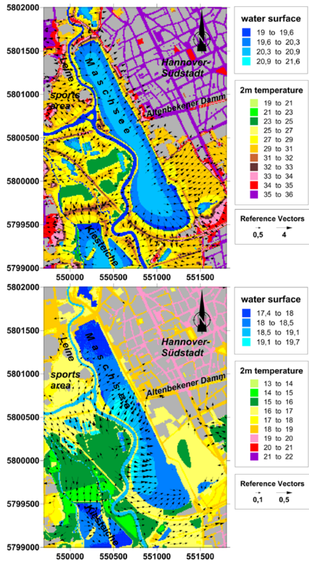
Figure 7: Simulated wind and temperature in 2m a.g. for daytime (above) and for night time (below). ❶ and ❷ indicate location of the observation sites.
