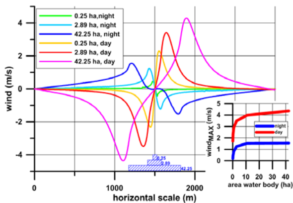
Figure 1: Simulated 10m wind for 14 hours (day) and 04 hours (night) for different water body areas (blue rectangles indicate location). Maximum wind speed for the two selected times depending on size of the pond is given in the inserted graph.
